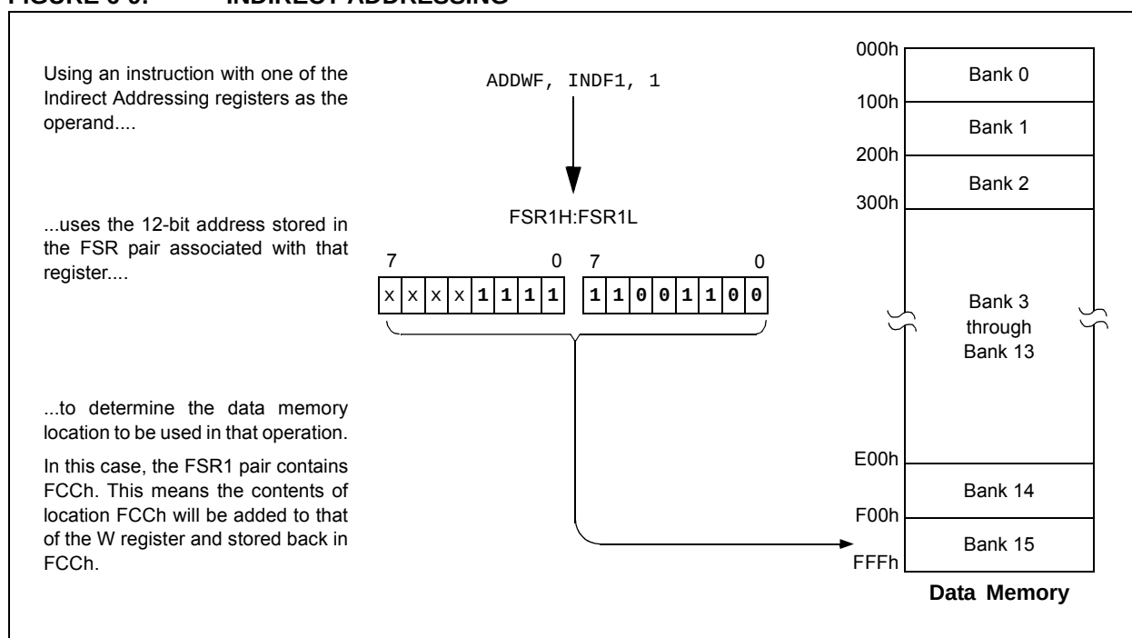
FIGURE 6-9: INDIRECT ADDRESSING
