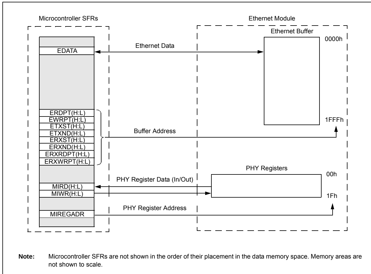
FIGURE 19-4: RELATIONSHIP BETWEEN MICROCONTROLLER AND ETHERNET MEMORY SPACES
